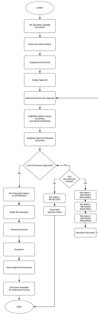
Figure 4.8: Document Approval Workflow
