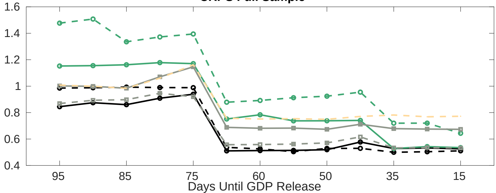
CRPS Full Sample
