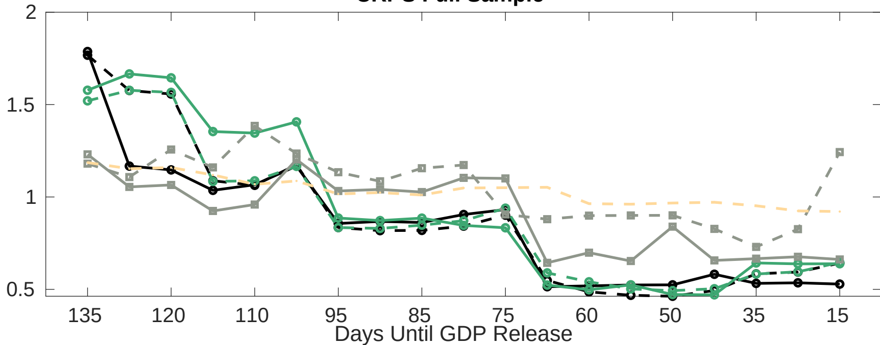
CRPS Full Sample
