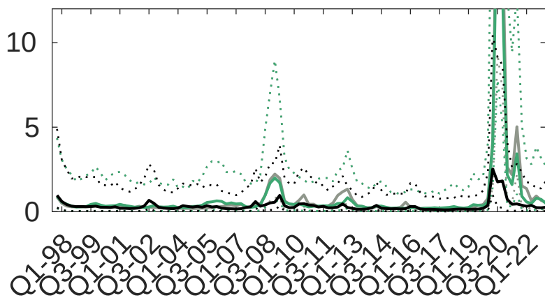
SV: Observation
