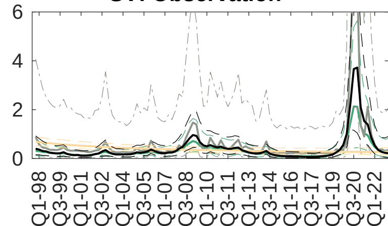
SV: Observation
