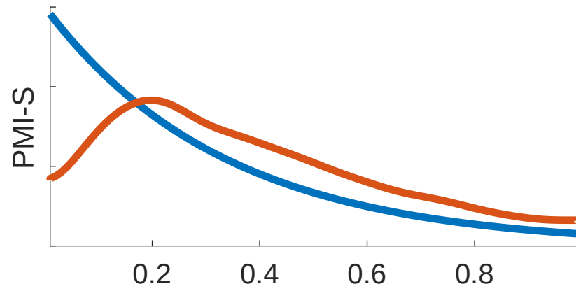
Nowcast Period 1
