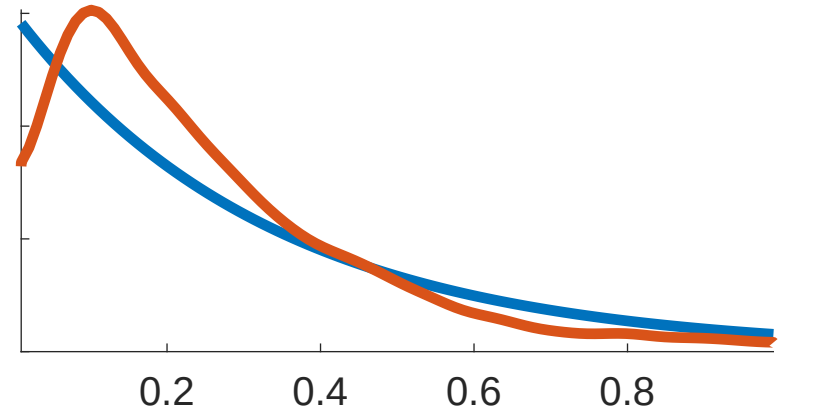
Nowcast Period 20
