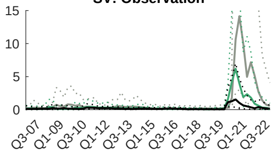
SV: Observation
