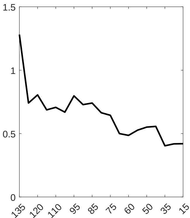
CRPS
