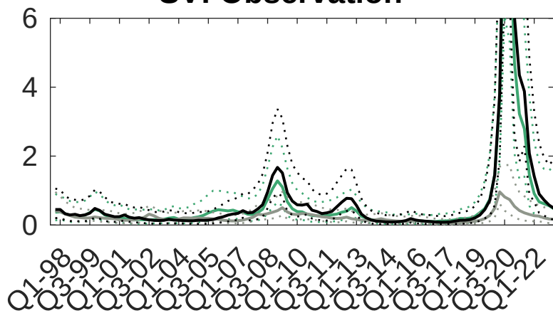
SV: Observation
