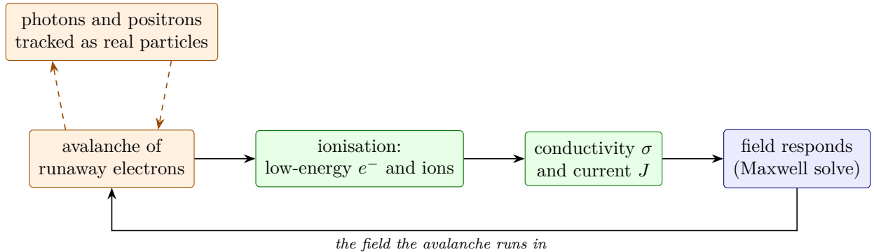
Figure 1: The loop that is closed here. Solid path: the avalanche creates a low-energy plasma, which conducts, which discharges the field, which changes the avalanche the field is driving. Dashed path (left arrow up, right arrow down): photons and positrons are produced by the avalanche and carried as kinetic species, so they can travel back upstream and seed new avalanches.
