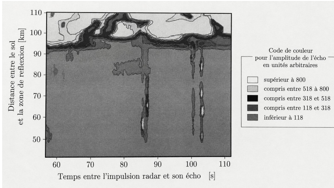
Figure 6: Map of ground-based radar echoes at 2.2 MHz for the event recorded at 13:39 on 15 October 1994 at the Korhogo station (Côte d'Ivoire). Figure taken from the article HF echoes from ionization potentially produced by high-altitude discharges , R. A. Roussel-Dupré and E. Blanc, Journal of Geophysical Research , vol. 102, no. A3, pp. 4613–4622, 1997.
