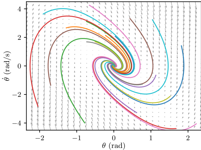
Closed-Loop Vector Field
