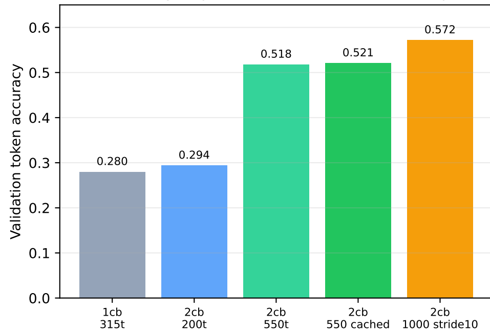
Accuracy improved with scale and cleanup
