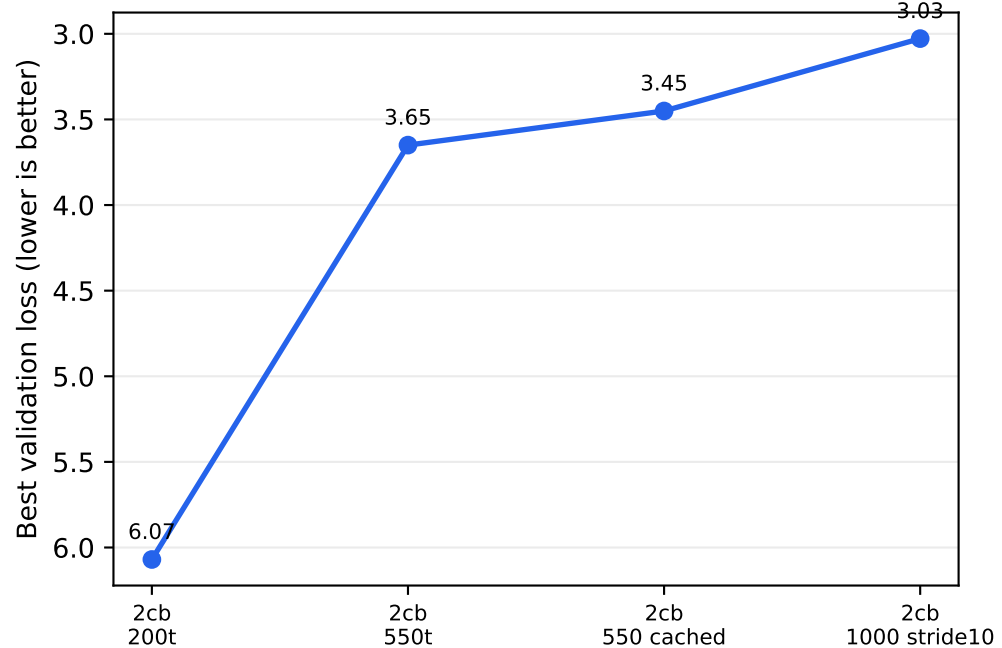
Best loss across main audio-token runs
