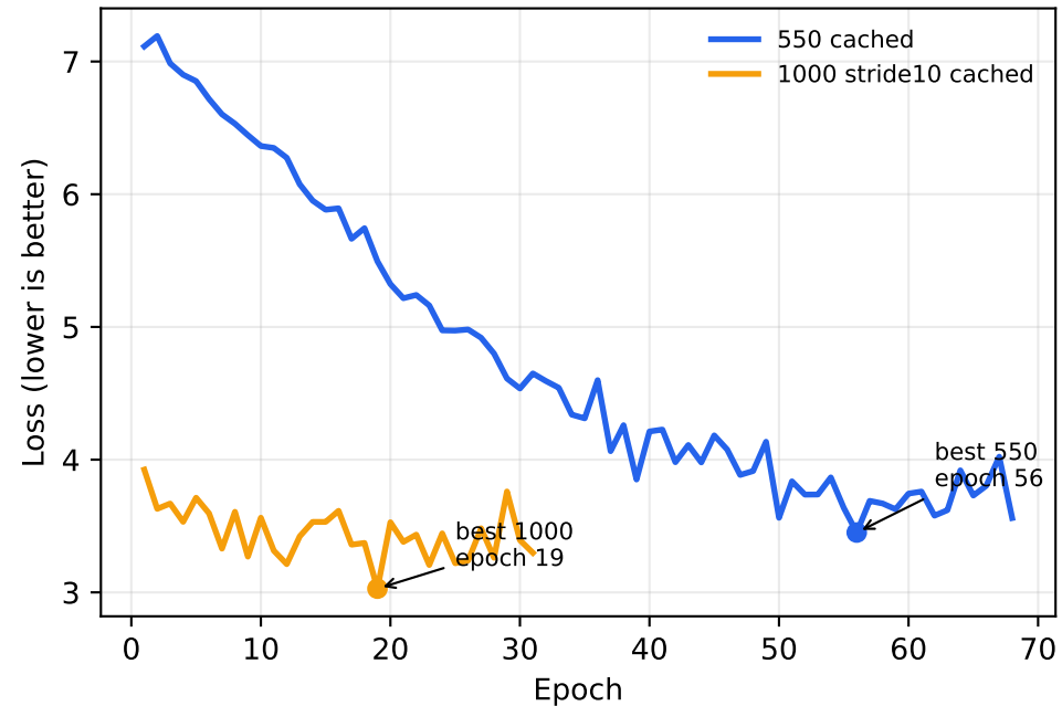
Validation loss
