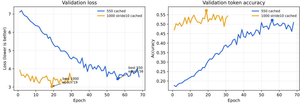
Figure 7: Validation loss and token accuracy curves for the two strongest cached audio-token runs. The 1000-track fixed-stride run starts from the 550-track checkpoint and reaches its best validation loss much earlier.
