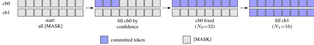
Figure 4: Coarse-to-fine mask-predict generation. The target starts as all mask tokens. Codebook 0 is filled first over N_0 = 32 iterations, committing the most confident positions at each step (the causal bias favors earlier time positions, drawn as a left-to-right fill); once codebook 0 is fixed, codebook 1 is filled over N_1 = 16 iterations conditioned on it. The decoded token tensor is then passed to EnCodec.
