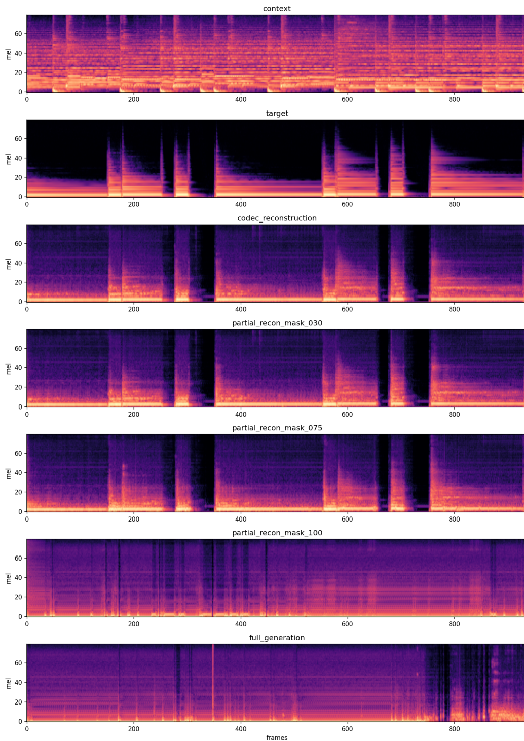
Figure 8: Mel-spectrogram diagnostic from a cached audio-token run. The important pattern is that codec and partial-mask reconstruction are more stable than full-mask generation.
