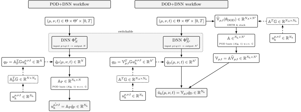
Figure 4.1: Dimensional workflow for POD+DNN (left) and DOD+DNN (right). Solid arrows show forward workflow and dashed arrows show training input
