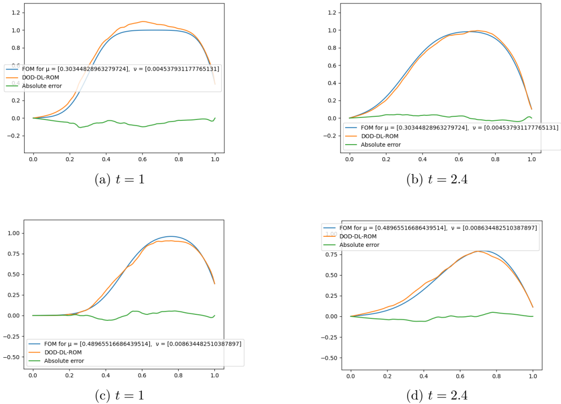
Figure 5.11: Two solutions of the DOD-DL-ROM
