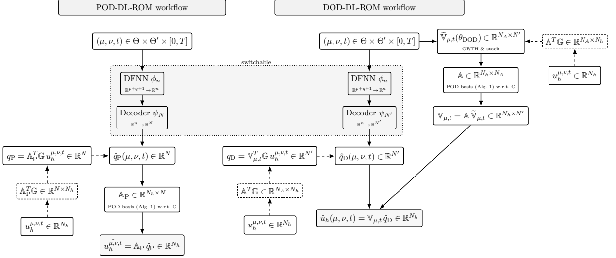
Figure 4.2: Dimensional workflow for POD-DL-ROM (left) and DOD-DL-ROM (right). Solid arrows show the forward calls; dashed arrows show pre-reduction of training data flow.
