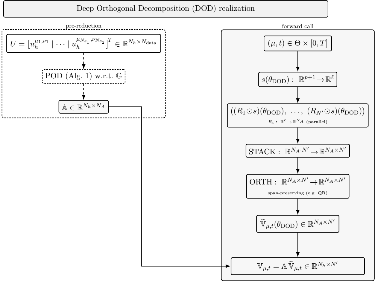
Figure 3.1: Realization of the Deep Orthogonal Decomposition for given \theta_{\text{DOD}} \in \Theta(\Phi_{\tilde{\mathbb{V}}})
