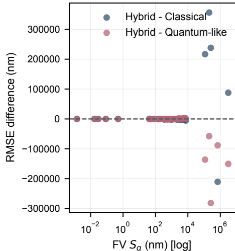
(c) Hybrid gain vs FV S_q
