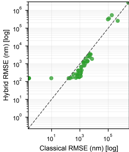
(a) Hybrid vs classical
