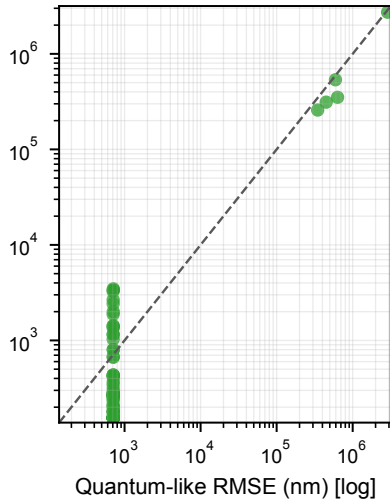
(b) Hybrid vs quantum-like
