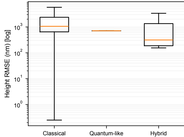
(a) RMSE distribution
