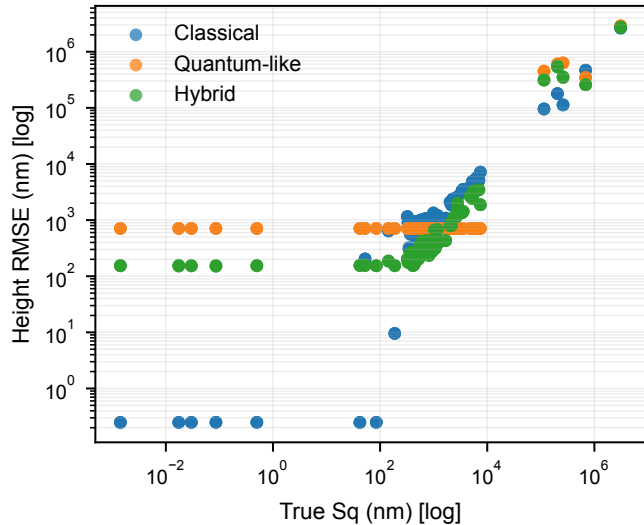
(b) RMSE vs roughness
