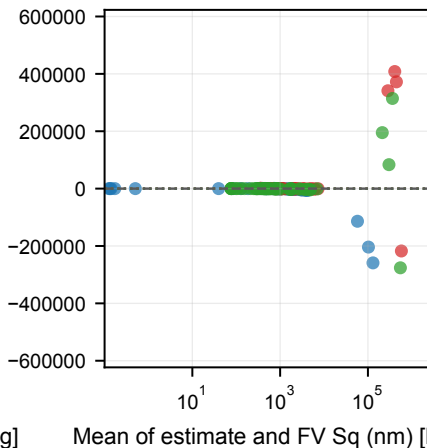
(Sq) Bias vs mean level
