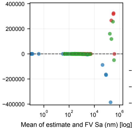
(Sa) Bias vs mean level
