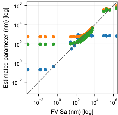
(Sa) Estimated vs FV reference
