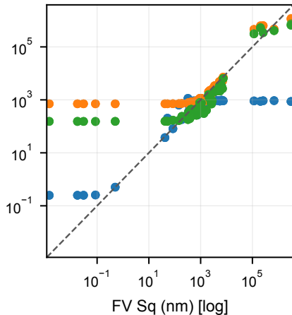
(Sq) Estimated vs FV reference
