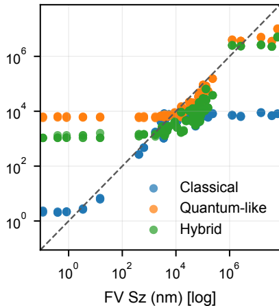
(Sz) Estimated vs FV reference
