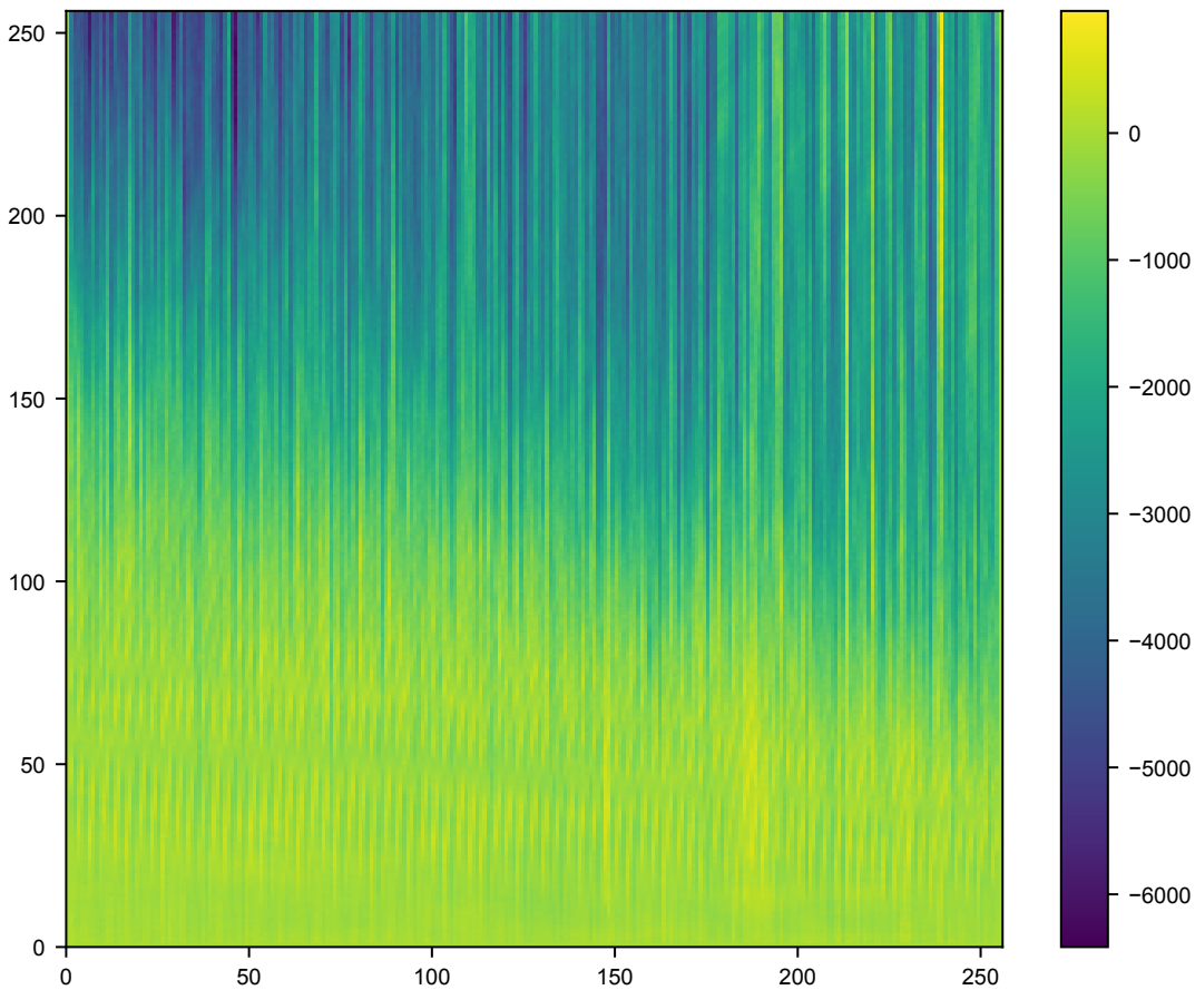
h_classical (nm)
