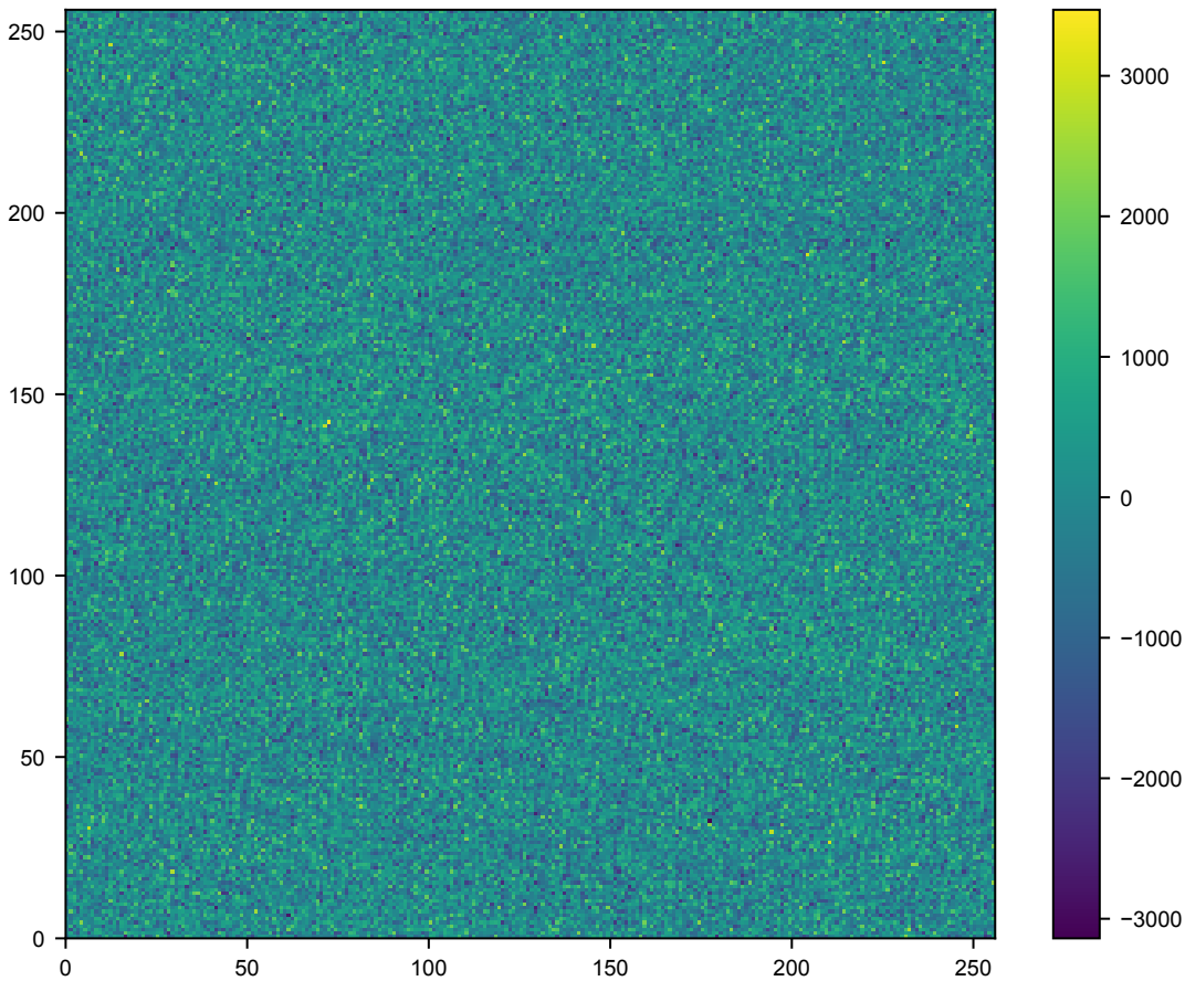
h_{\text{quantum-like}} (nm)
