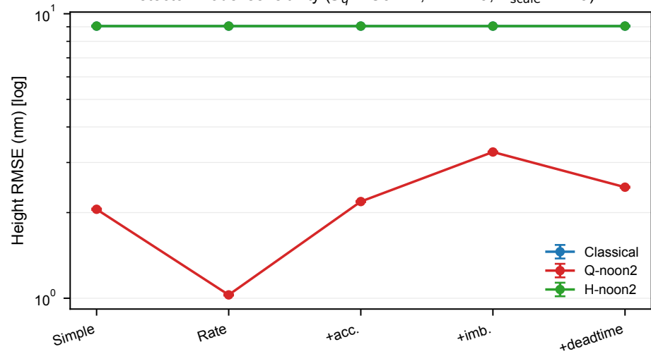
Detector-model sensitivity ( S_q = 80 nm, R = 1.0 , V_{\text{scale}} = 1.0 )
