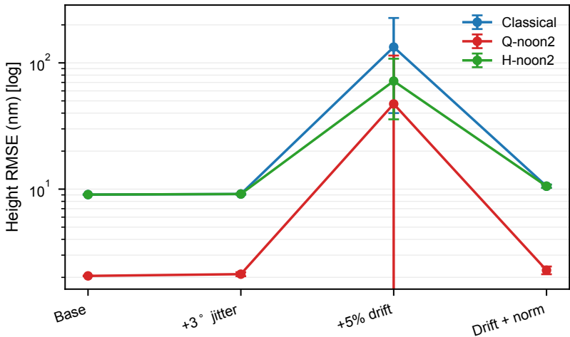
Representative non-ideality stress test ( S_q = 80 nm, R = 1.0 , V_{\text{scale}} = 1.0 )
