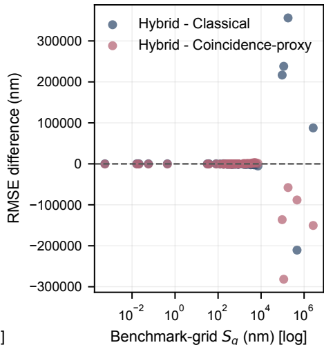
(c) Hybrid gain vs benchmark-grid S_q
