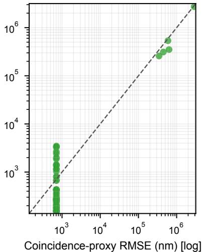
(b) Hybrid vs coincidence-proxy
