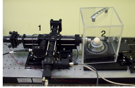
Figure 2: The complete measurement system: (1) modified Michelson interferometer in cage mounting, (2) high-precision rotation stage with the artefact.
