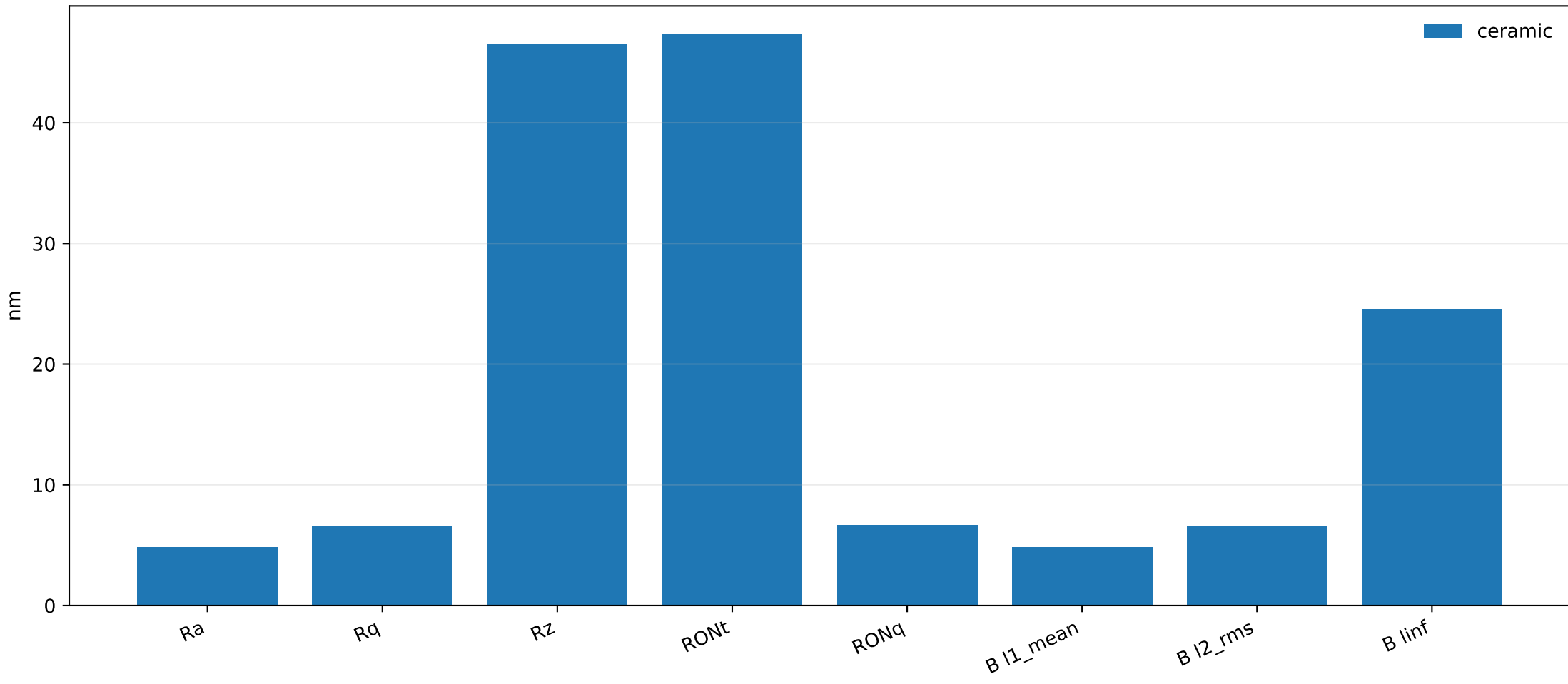
Classical profile/roundness and Banach descriptors from radial EFM profiles
