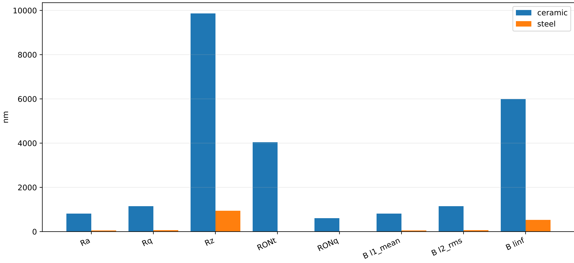
Profile-style and Banach descriptors from reconstructed height
