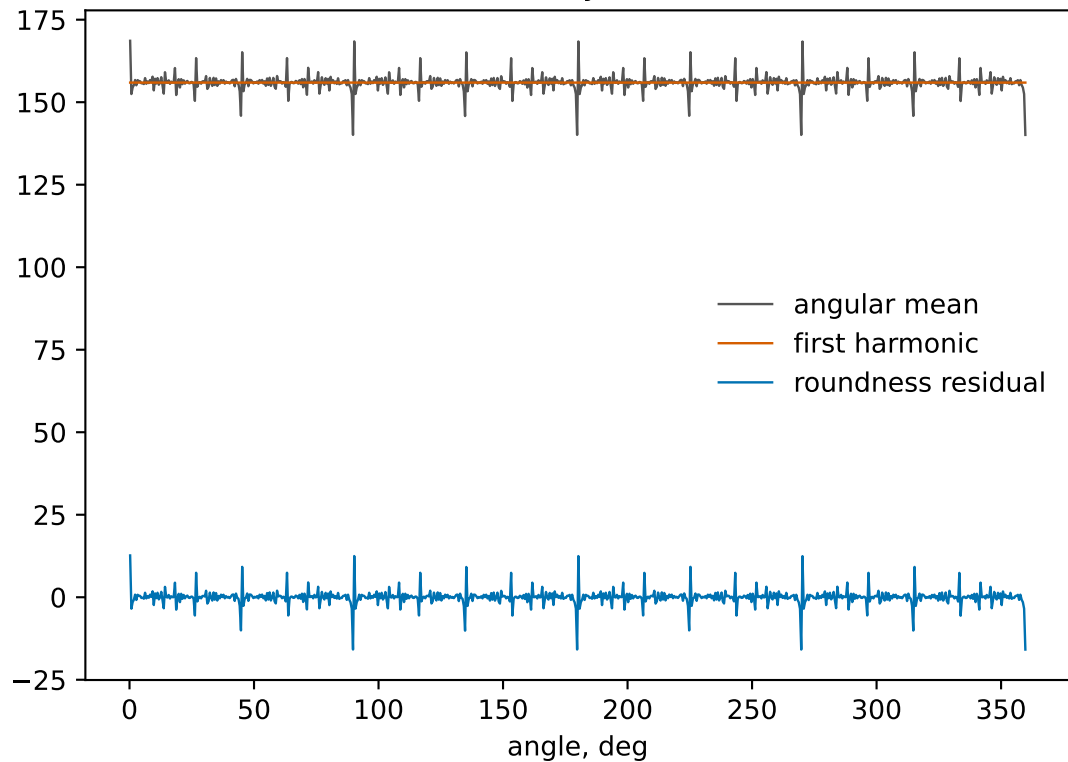
Eccentricity removal
