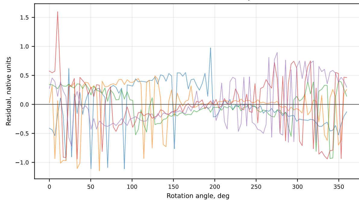
Roundness deviation after eccentricity removal
