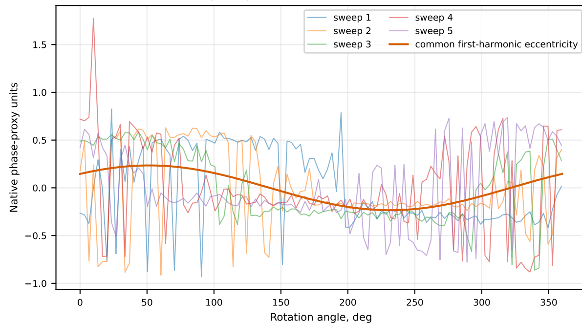
Eccentricity component fitted before roundness evaluation
