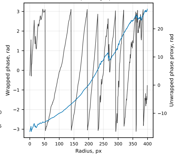
Radial phase graph
