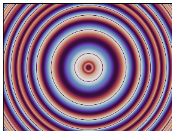
Wrapped phase proxy, full -\pi..pi scale
