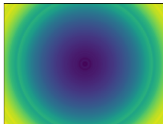
Unwrapped phase proxy, full scale
