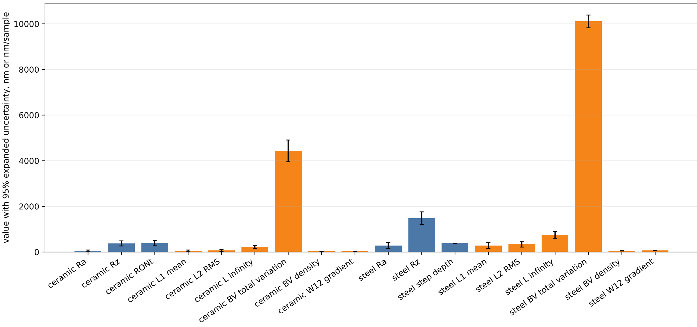
ISO/profile metrics versus Banach descriptors with sweep-repeatability uncertainty
