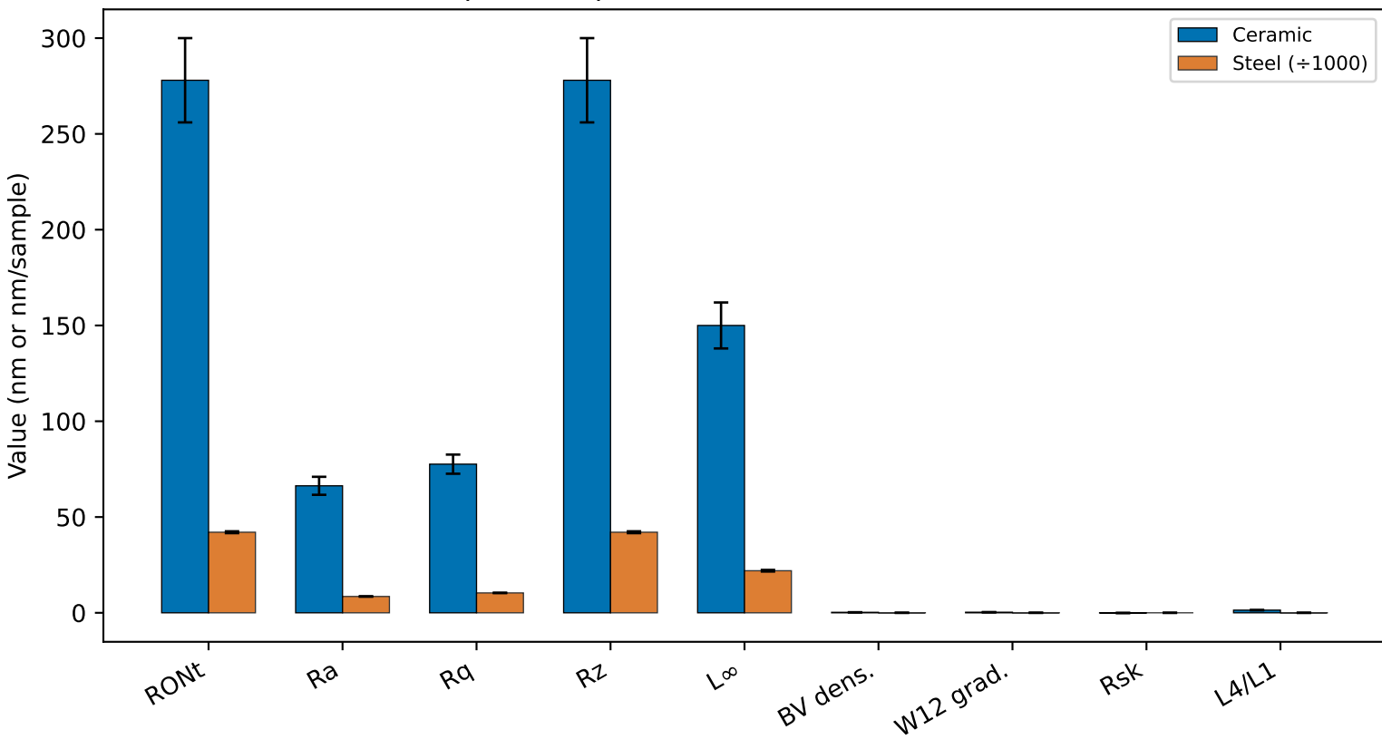
Descriptor comparison with U95 (LSCI + 0-15 UPR)
