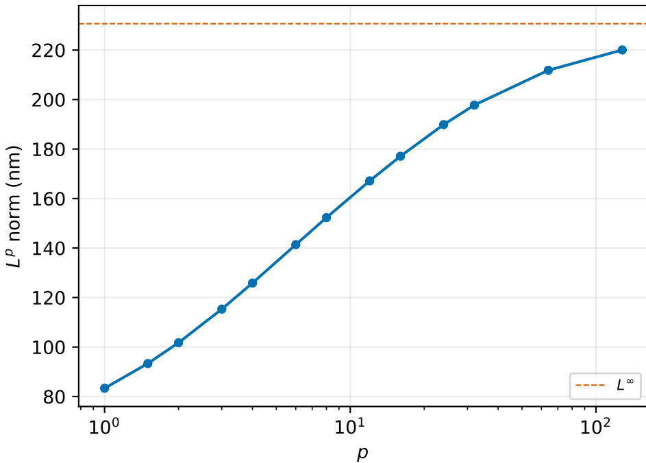
L^p norm convergence (ceramic)
