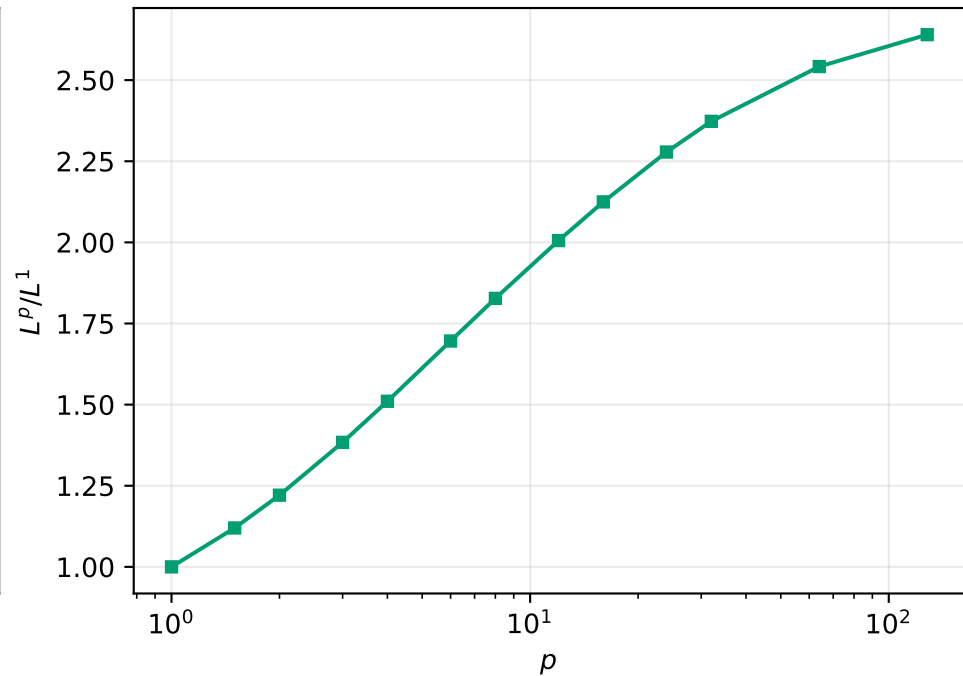
Peakiness ratio L^p/L^1
