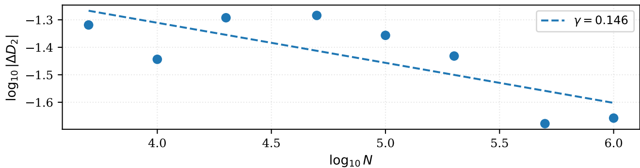
Power-law fit: |\Delta D_2| \propto N^{-\gamma} (primes only)
