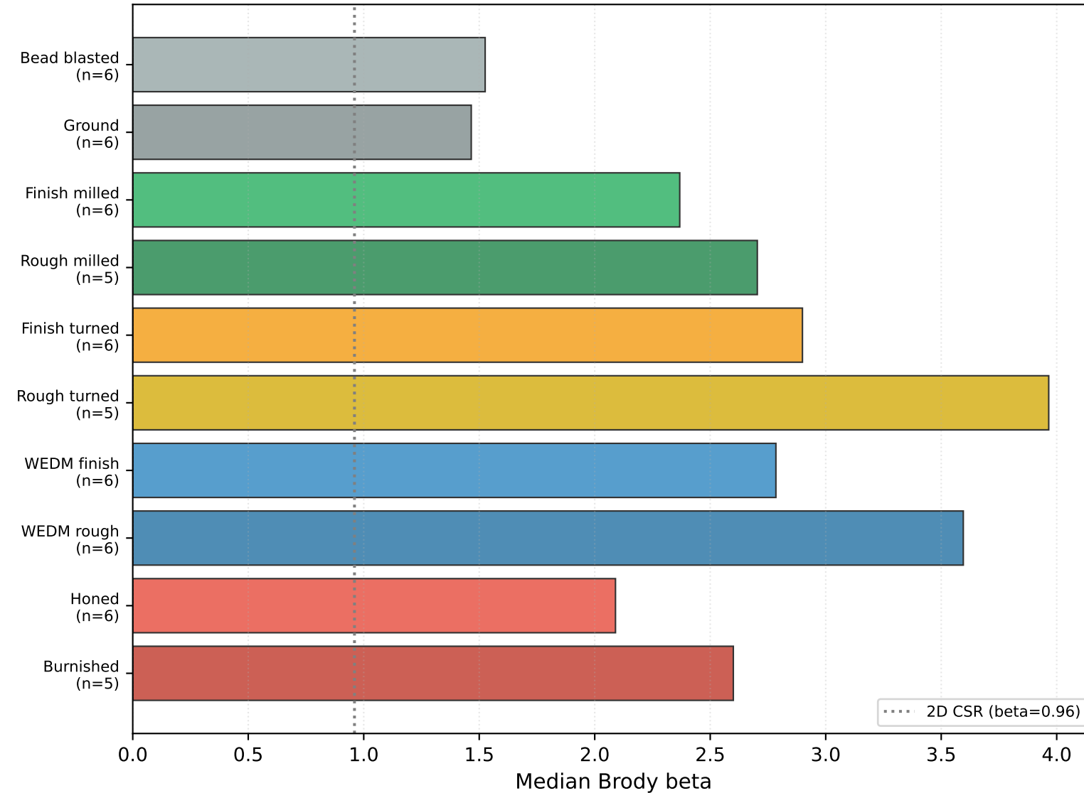
beta by manufacturing process
