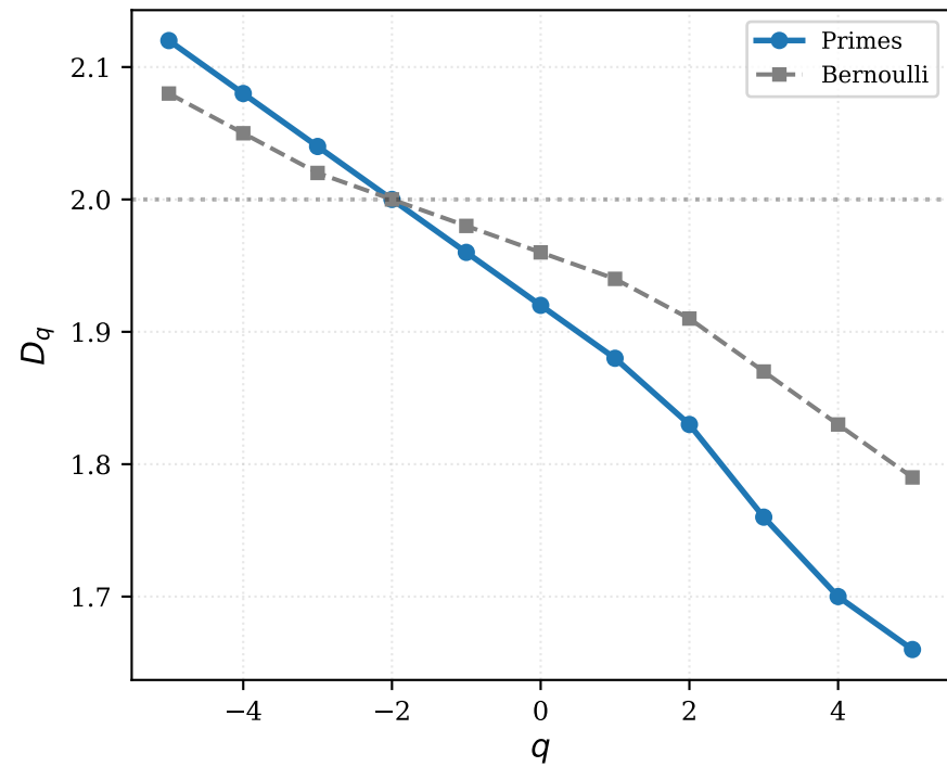
D_q spectrum
