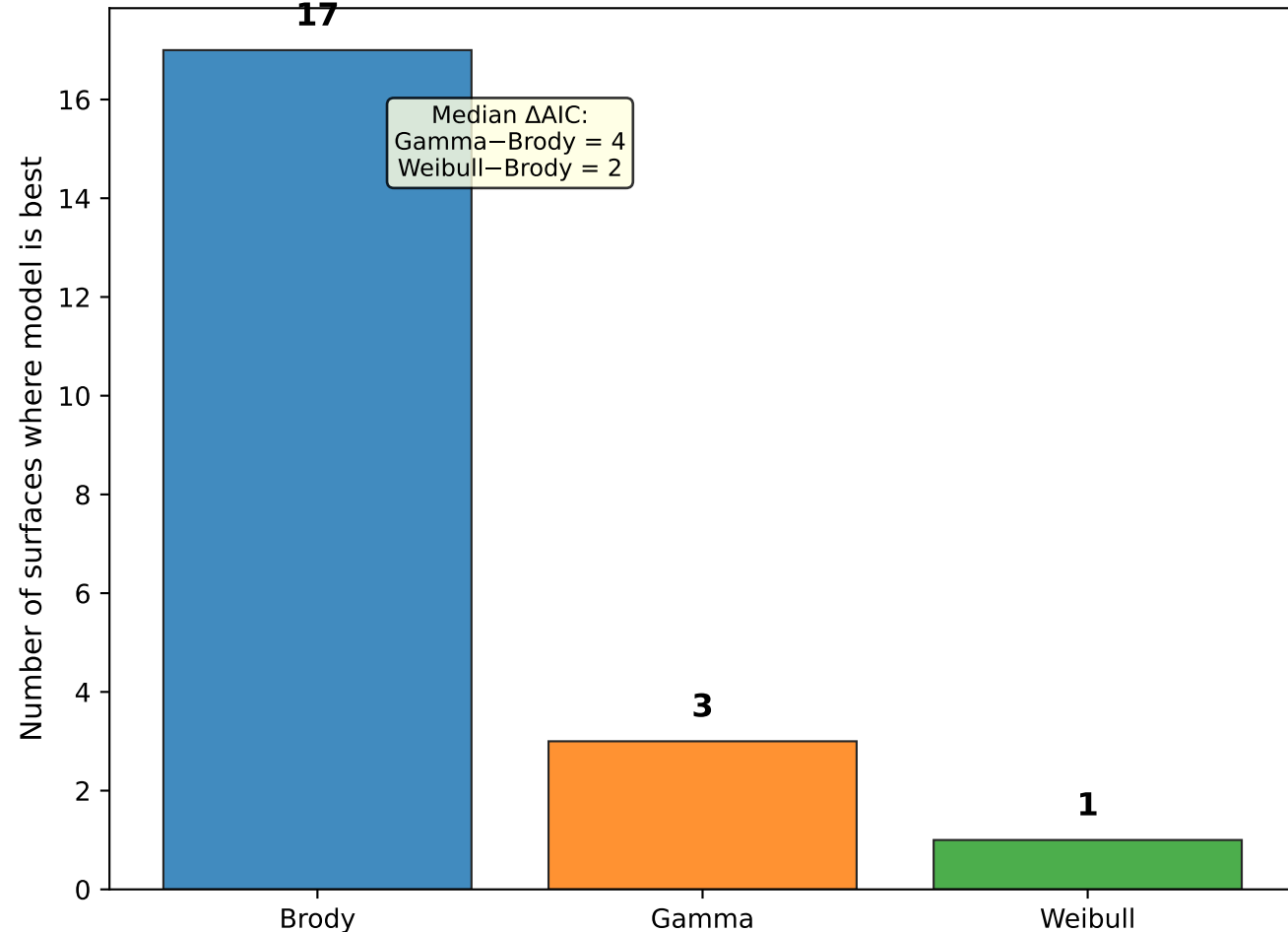
(b) AIC comparison (n=21 surfaces)
