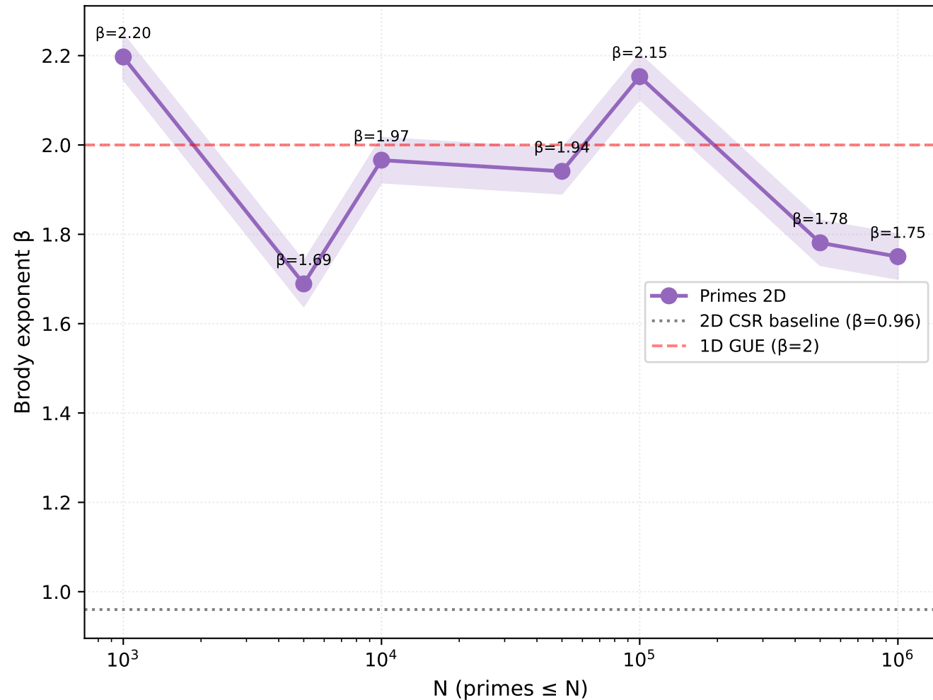
(a) Prime \beta(N) convergence
