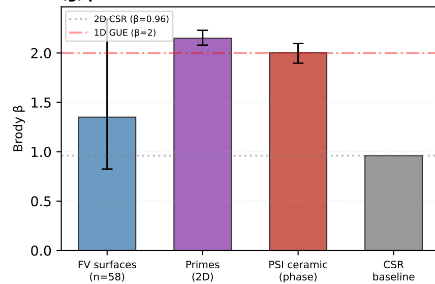
(g) \beta across domains
