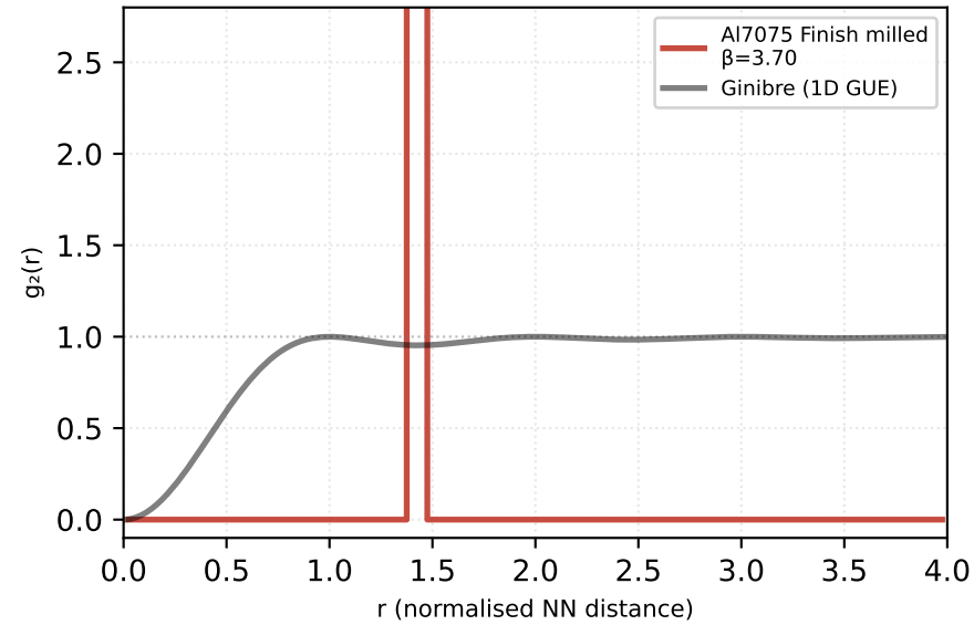
(a) Super-GUE ( \beta > 2 )
