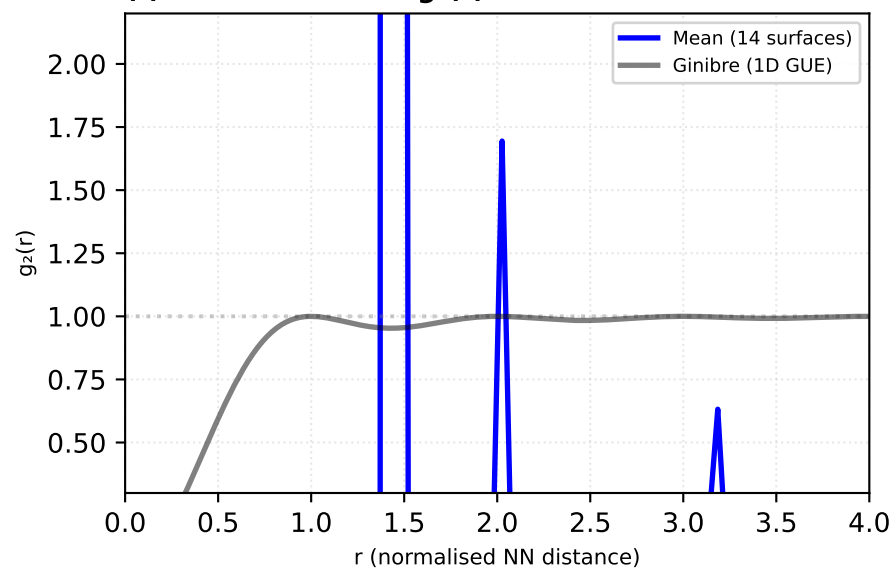
(f) Ensemble mean g_2(r)
