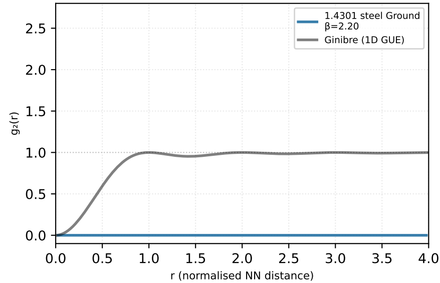
(b) GUE-like ( \beta \approx 2 )
