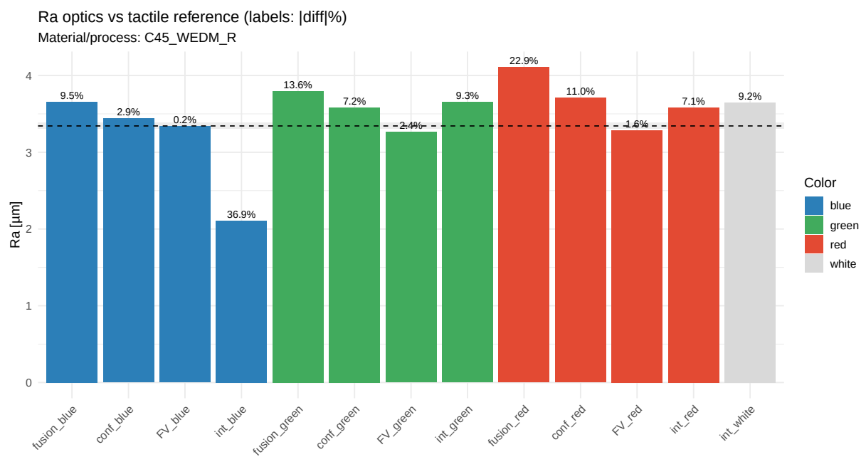
Figure S4: R_a : optical-tactile comparison for C45 after wire EDM rough cutting (single-pass), summarising relative disagreement across systems
