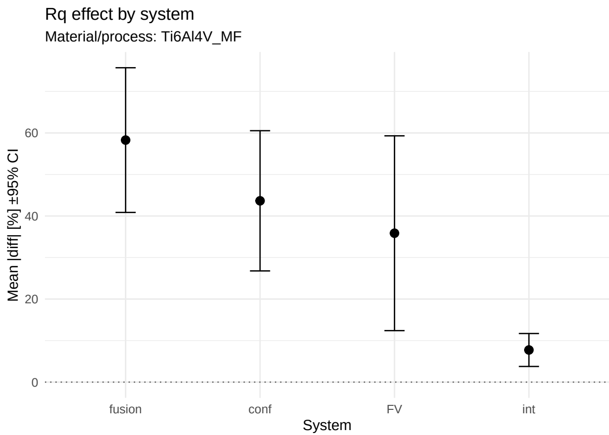
Figure S1: R_q : main effects of system on |diff|(\%) for Ti6Al4V after finish milling
