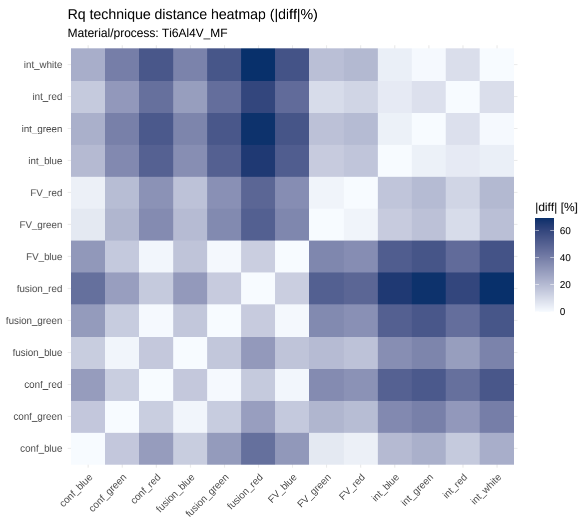
Figure S3: R_q : technical-distance heatmap between systems for Ti6Al4V after finish milling, based on mean |diff| (%)
