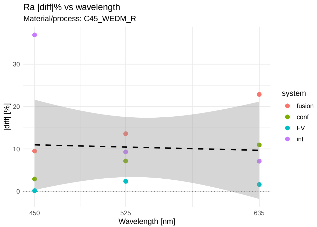
Figure S5: R_a : |diff| (%) versus illumination wavelength for C45 after wire EDM rough cutting (single-pass) with fitted screening lines
