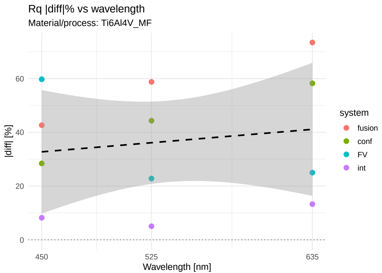
Figure S2: R_q : |diff| (%) versus illumination wavelength for Ti6Al4V after finish milling with fitted screening lines
