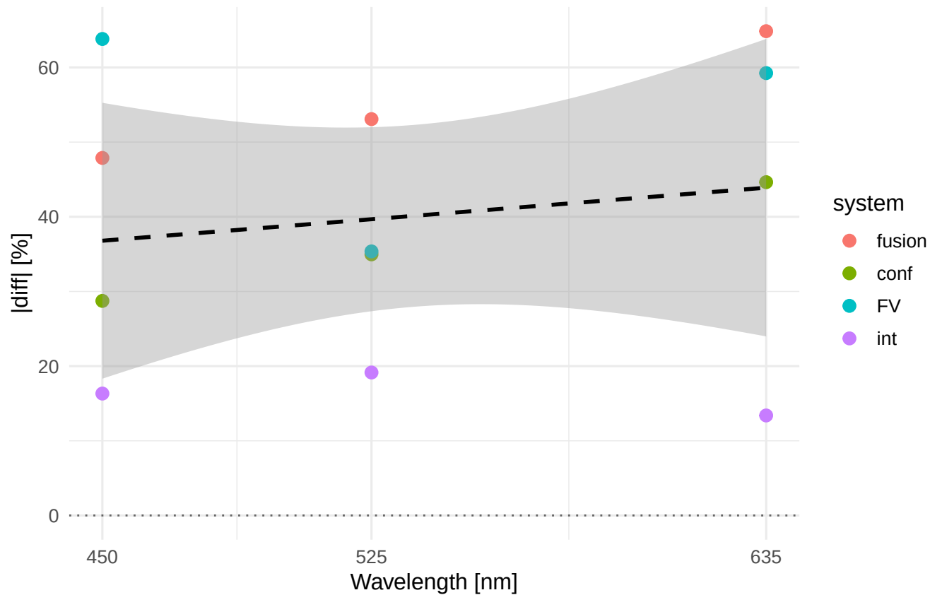
Ra |diff|% vs wavelength Material/process: 14301_GRI
