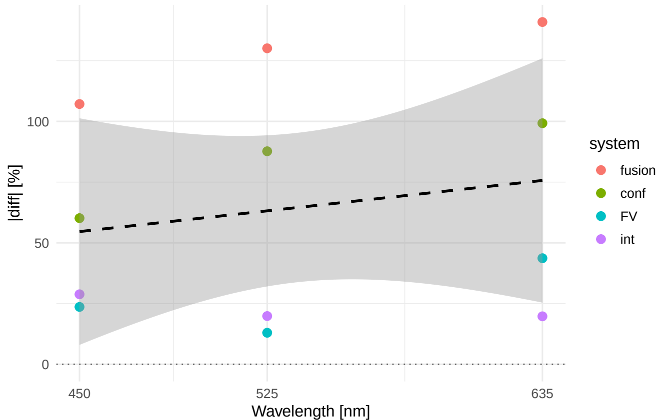
Ra |diff|% vs wavelength Material/process: C45_WEDM_F
