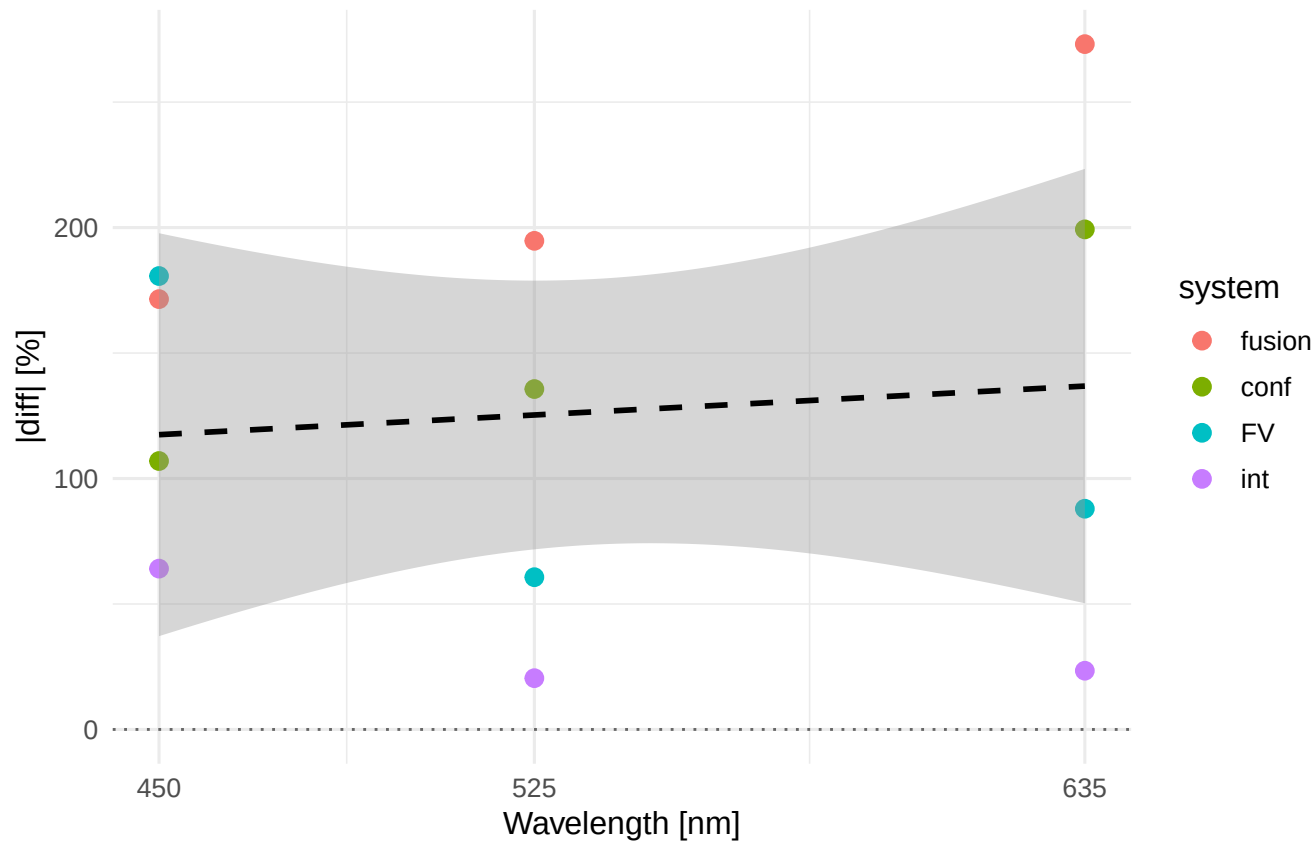
Ra |diff|% vs wavelength Material/process: ELLOR_HON
