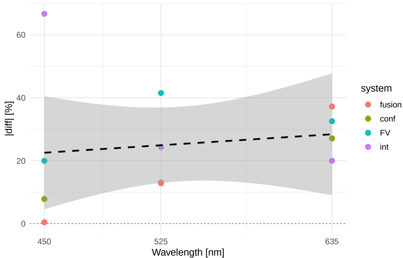
Ra |diff|% vs wavelength Material/process: ELLOR_MF
