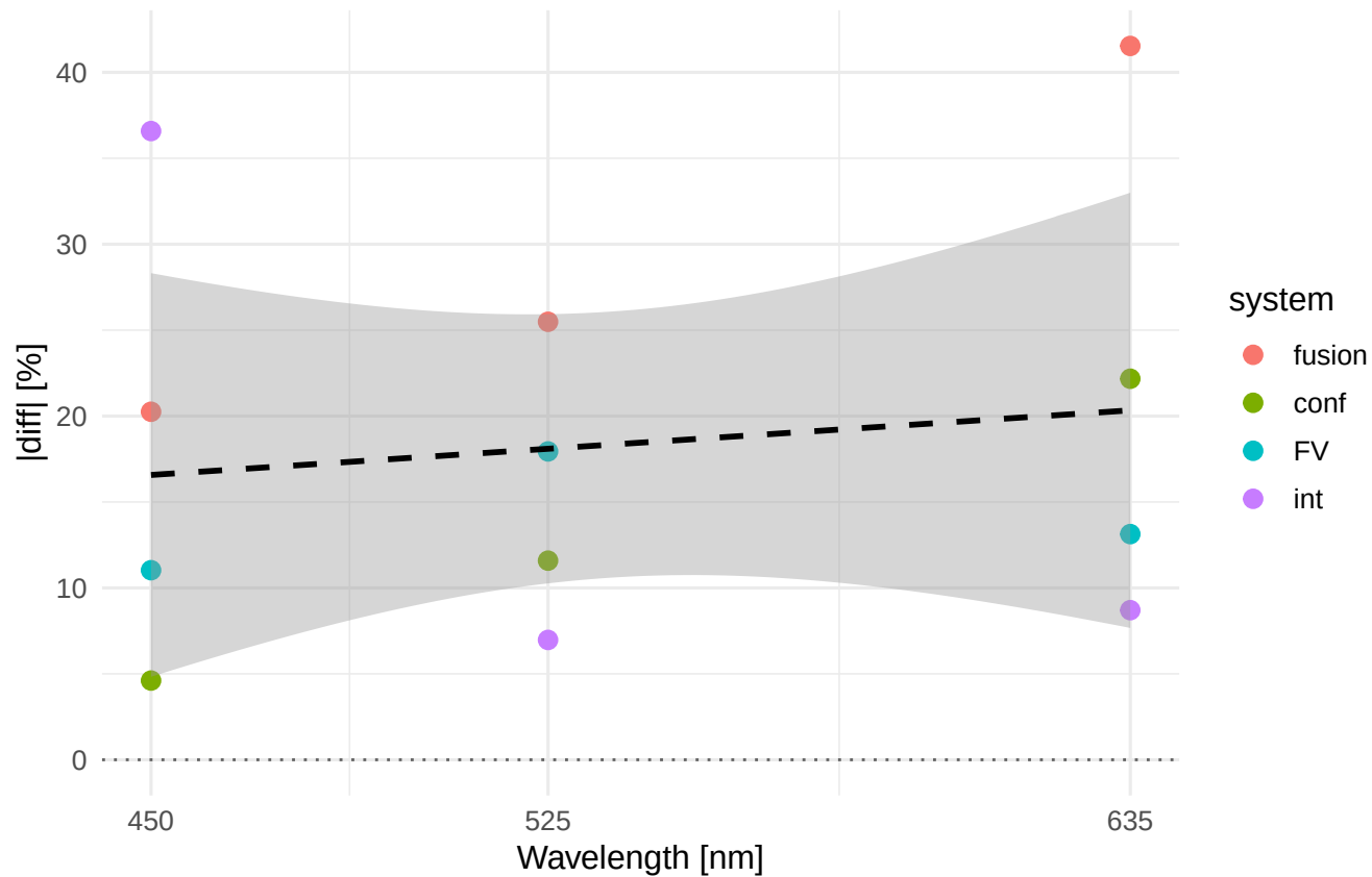
Ra |diff|% vs wavelength Material/process: ELLOR_TF
