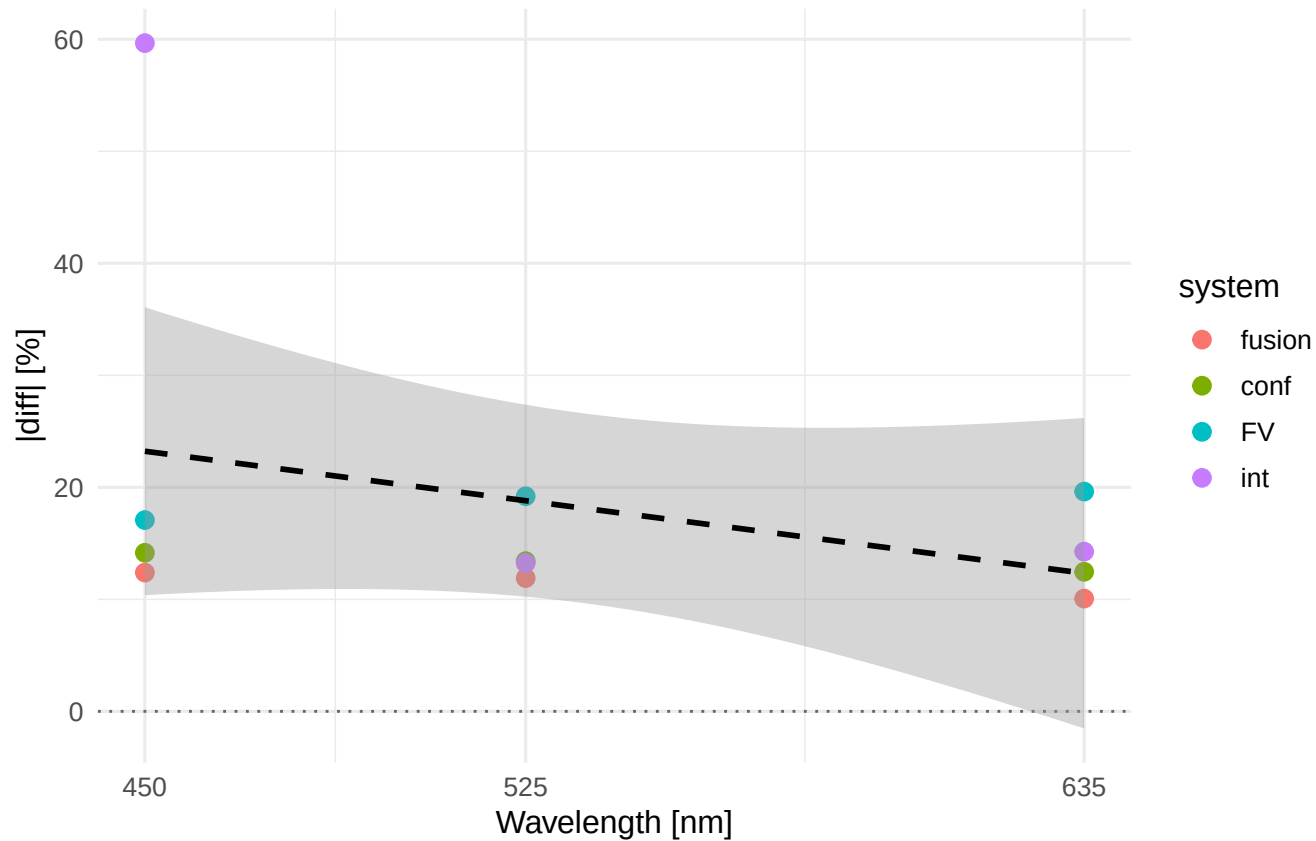
Ra |diff|% vs wavelength Material/process: ELLOR_TR
