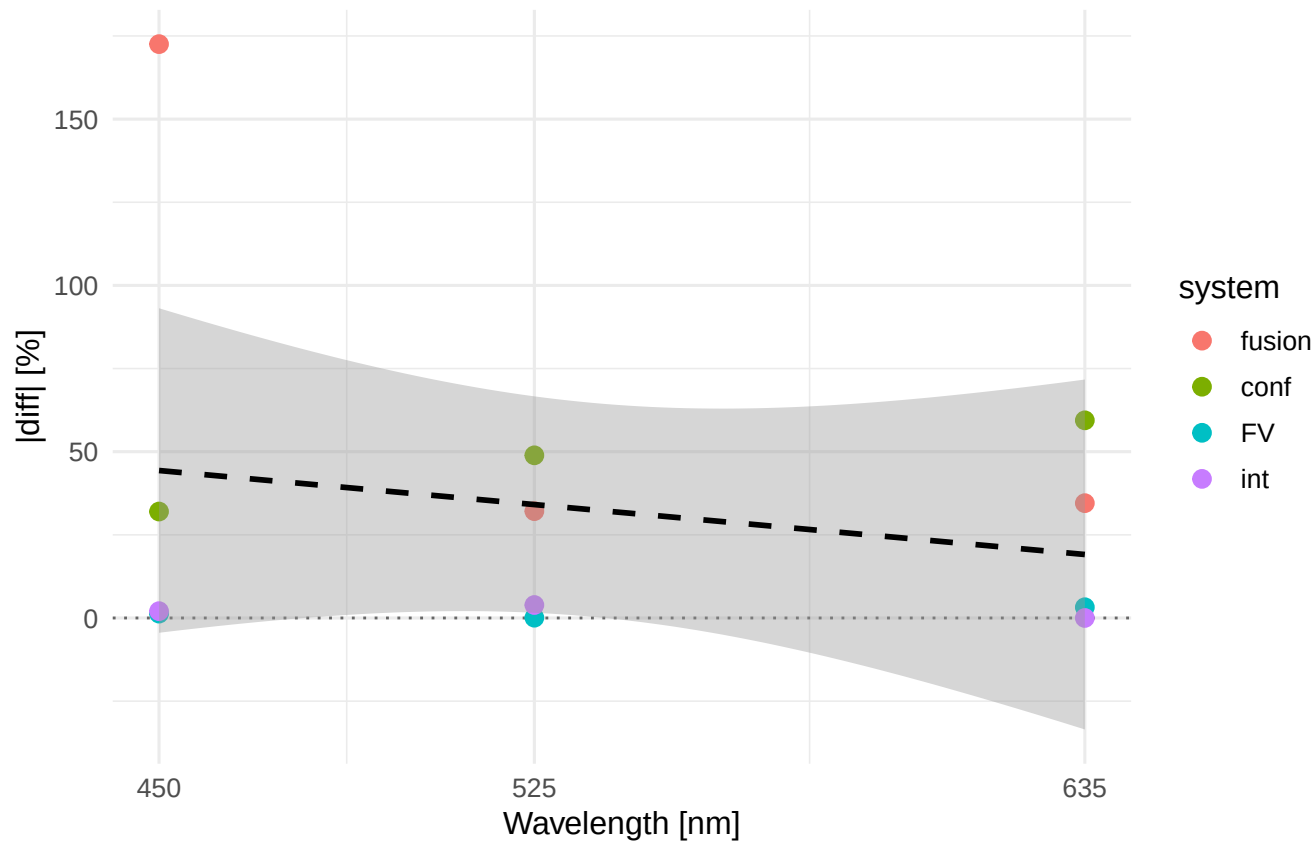
Rku |diff|% vs wavelength Material/process: C45_WEDM_F
