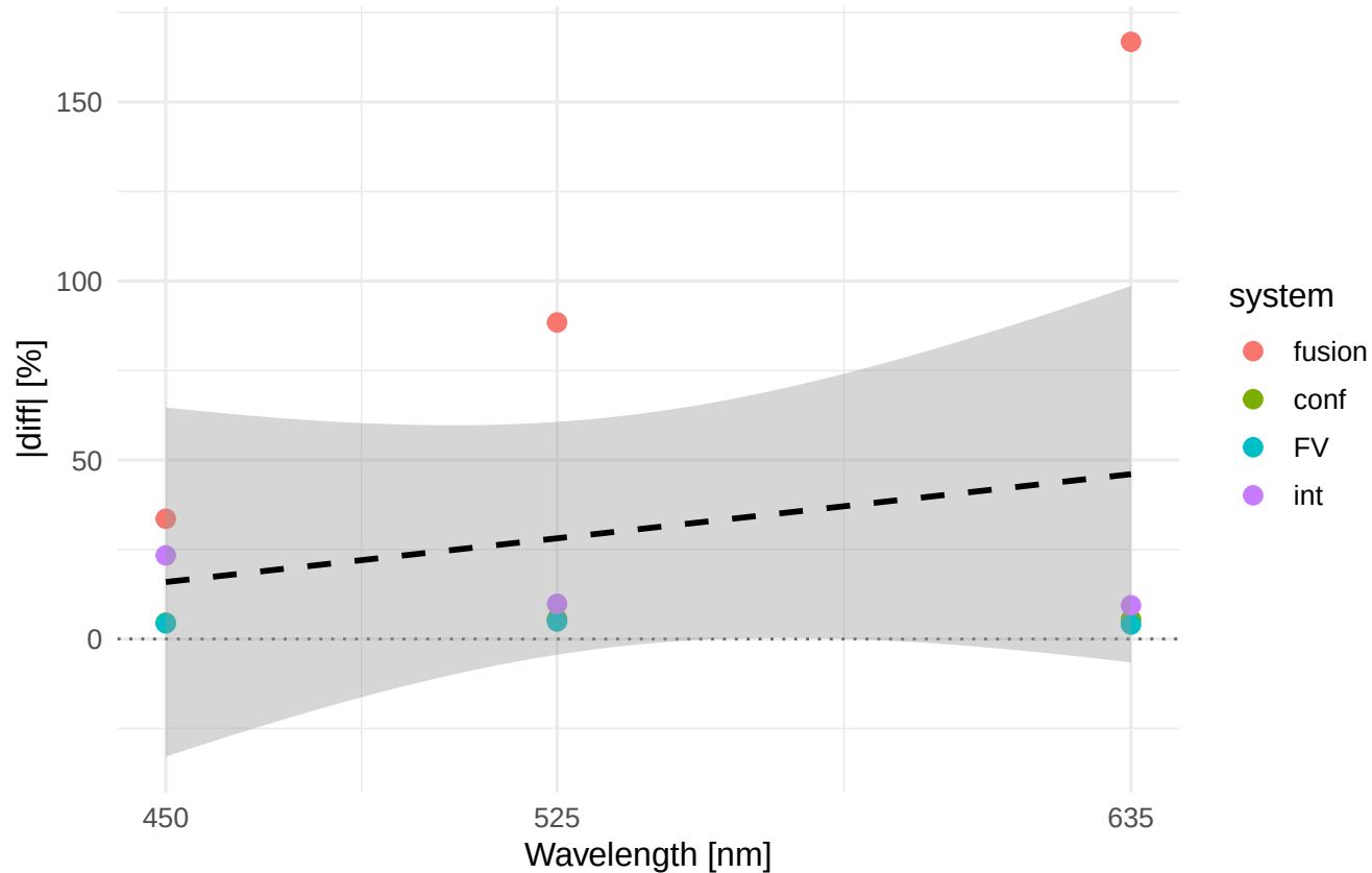
Rku |diff|% vs wavelength Material/process: C45_WEDM_R
