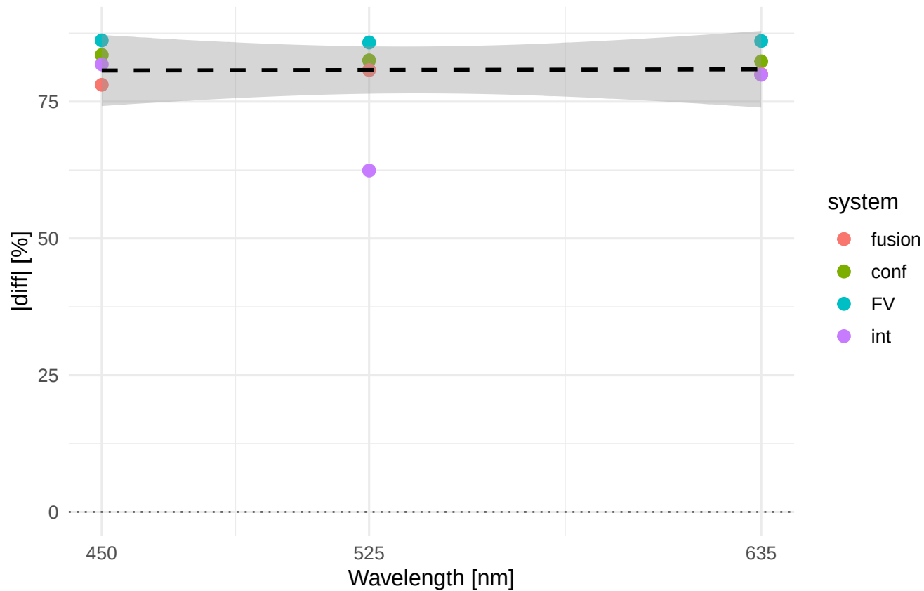
Rku |diff|% vs wavelength Material/process: ELLOR_HON
